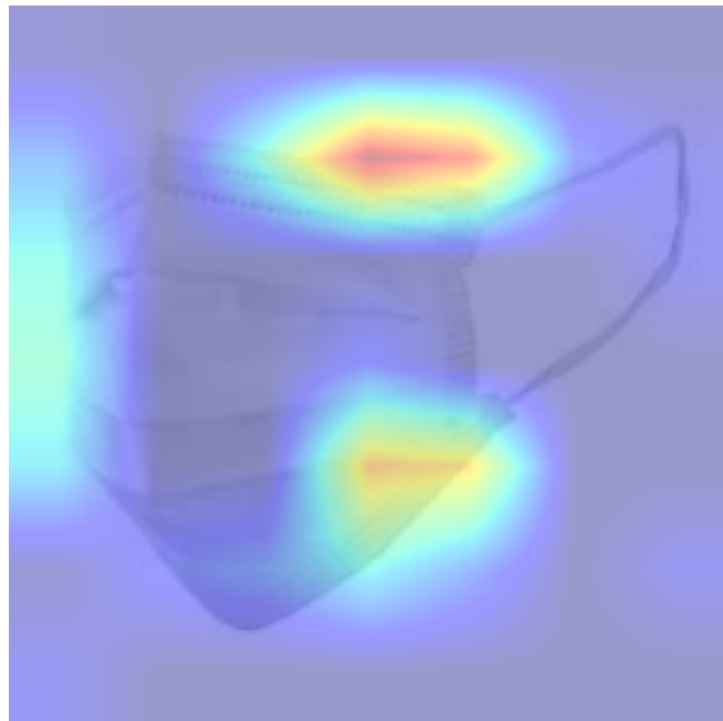
resnet50 Grad-CAM Confidence: 0.96
