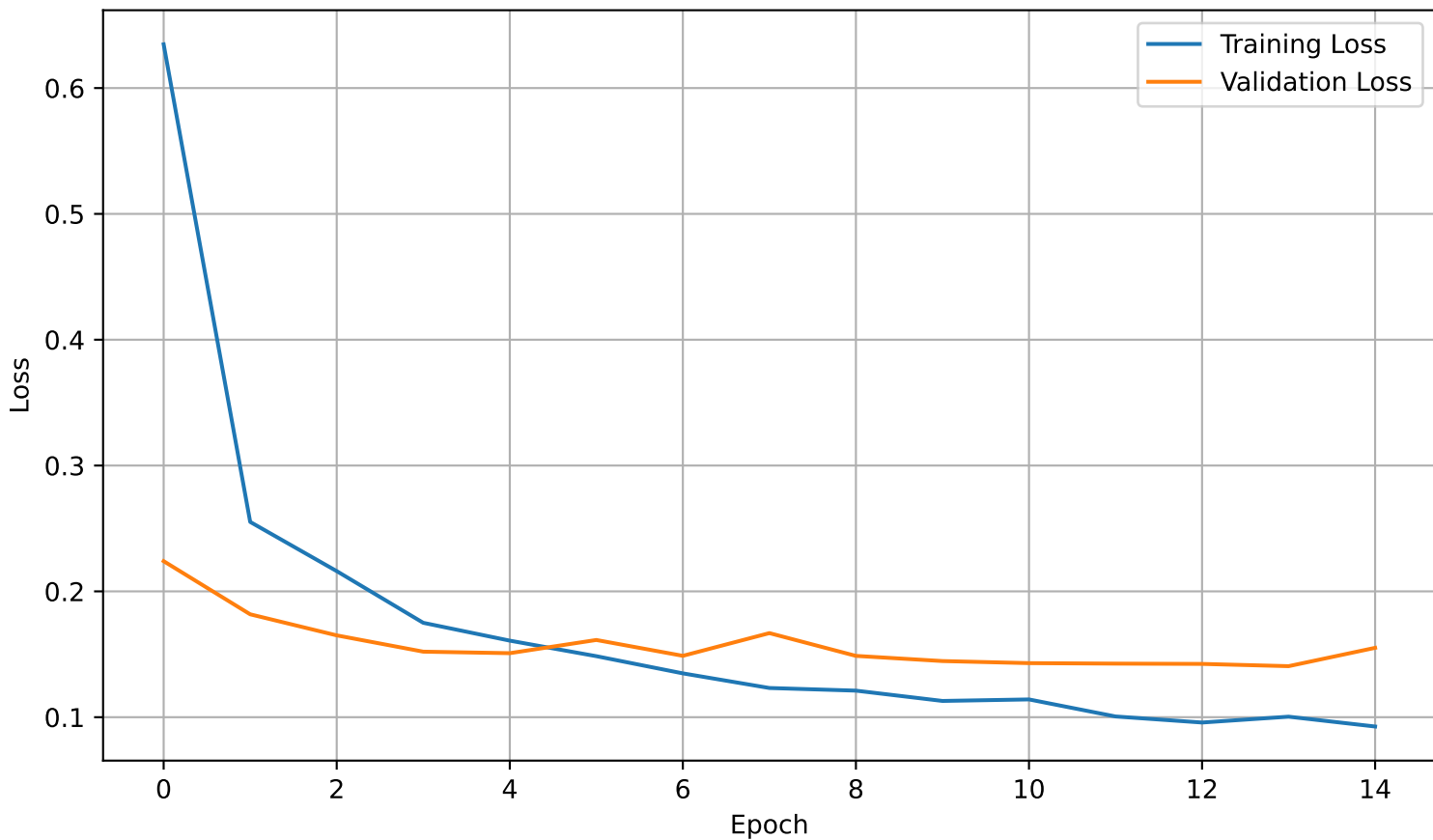
resnet50 Loss Curve
