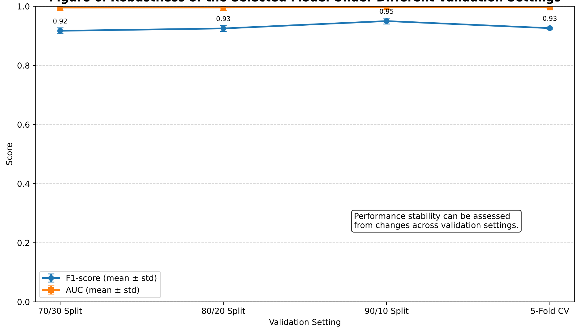
Figure 6. Robustness of the Selected Model Under Different Validation Settings
