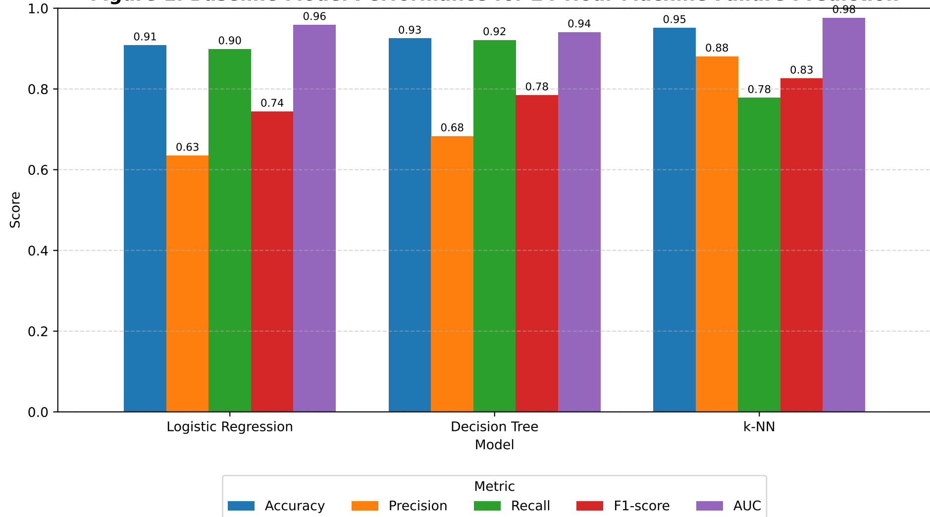
Figure 1. Baseline Model Performance for 24-Hour Machine Failure Prediction
