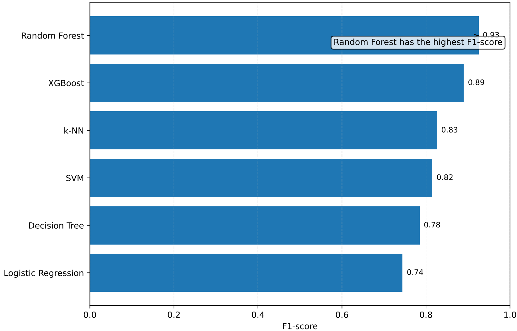
Figure 2. Overall Model Ranking for 24-Hour Machine Failure Prediction
