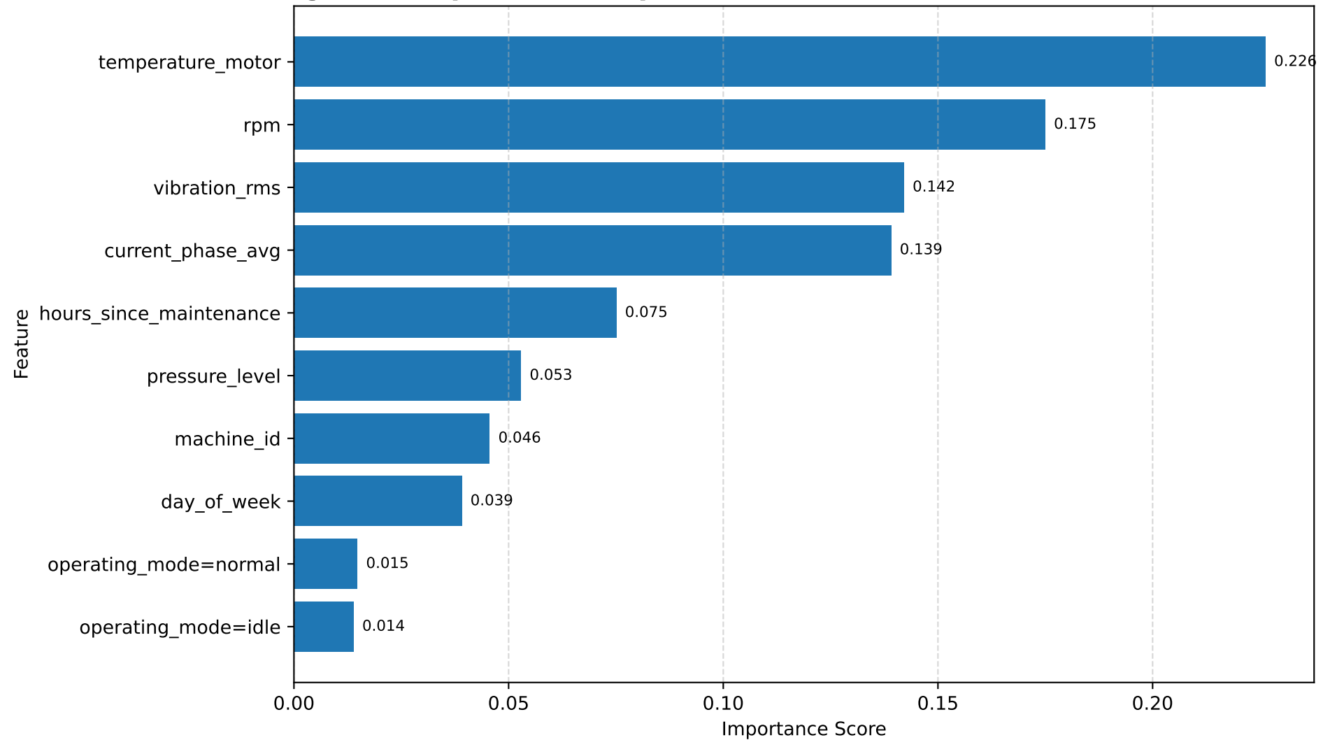
Figure 4. Top Feature Importance Scores for Machine Failure Prediction
