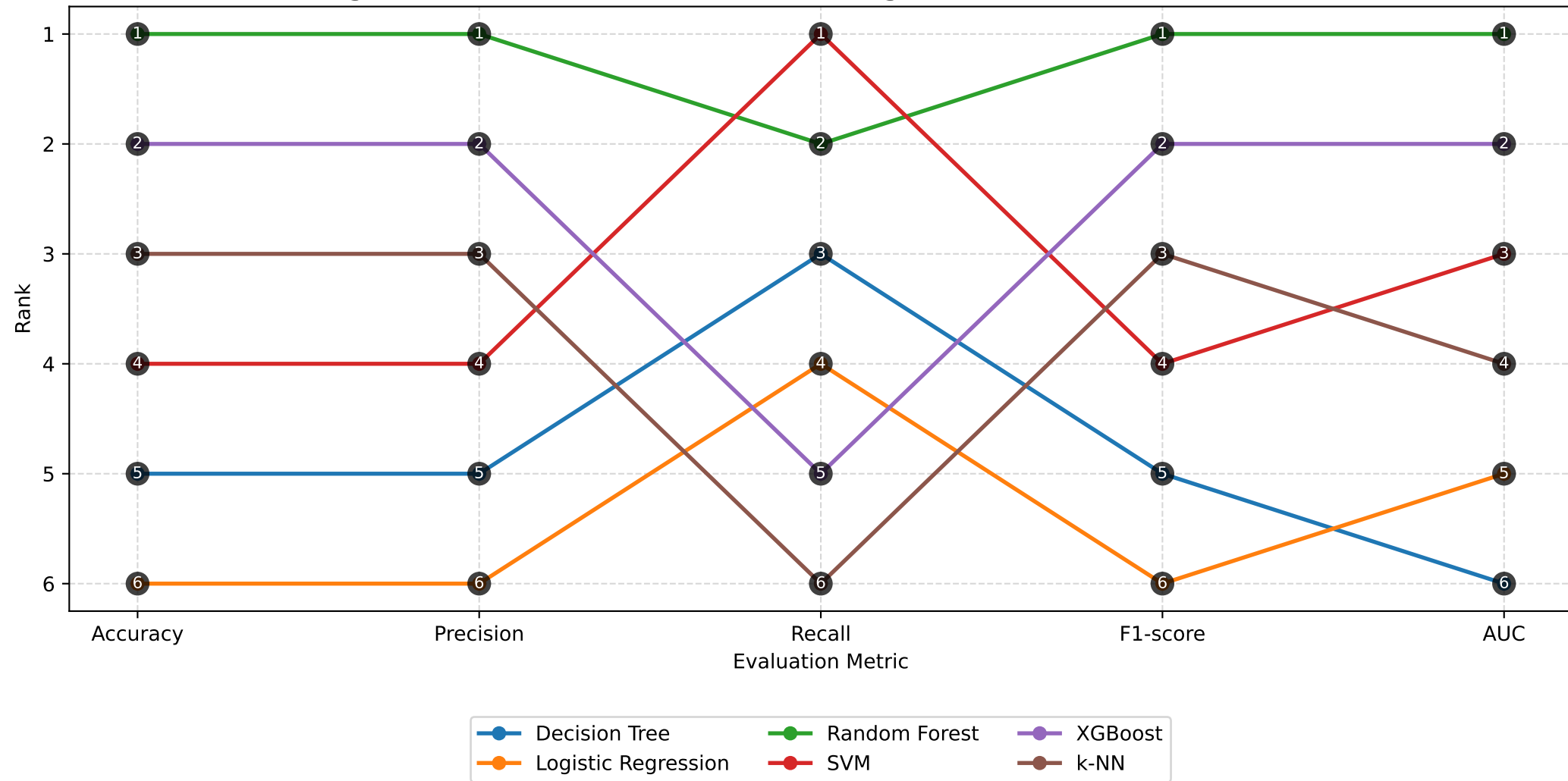
Figure 5. Variation in Model Ranking Across Evaluation Metrics
