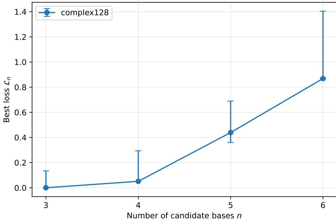
Multi-seed AMUB loss summary in d = 6
