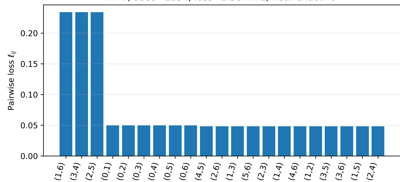
d6_n7_complex128_seed1234 n=7, seed=1234, loss=1.584472, near-exact=0
