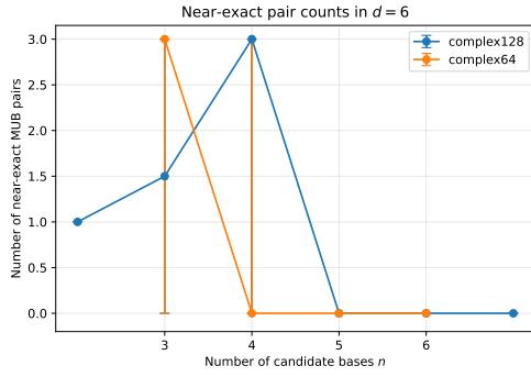
Figure 4: Near-exact MUB pair counts in d = 6 . This plot shows the median number of near-exact MUB pairs with corresponding ranges across five seeds. Near-exact pairs disappear for n \geq 5 under the primary tolerance, coinciding with a transition to fully defective observed configurations.
