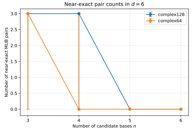
Figure 5: Near-exact MUB pair counts in d = 6 . The plot shows the median number of near-exact pairs with min-max ranges across 100 seeds. Under the primary tolerance, no near-exact pairs are observed for n = 5 or n = 6 in either precision.
