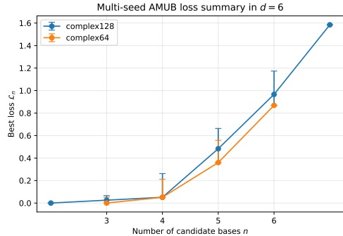
Figure 3: Best AMUB loss summary in d = 6 . This plot shows the median best loss with min–max range across five seeds. The AMUB loss increases with n .
