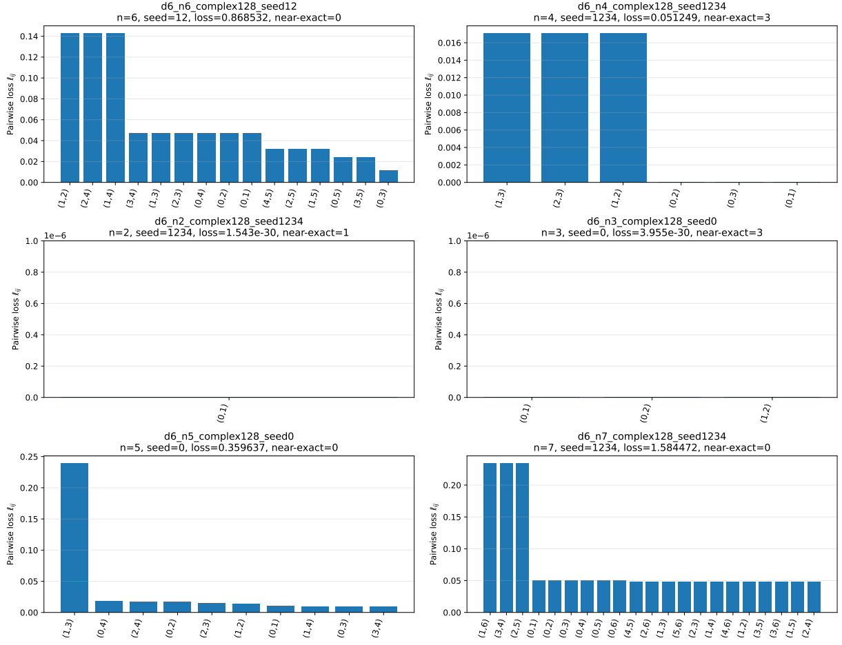
Figure 5: Sorted pairwise AMUB loss spectra for representative complex128 configurations. Each bar corresponds to one pairwise contribution \ell_{ij} . The exact n = 3 representative has pairwise losses at numerical zero, the defective n = 3 representative has three approximately equal nonzero losses, the n = 4 representative exhibits three near-zero losses and three equal defective losses, and the n = 5 and n = 6 representatives have no zero pairwise losses.
