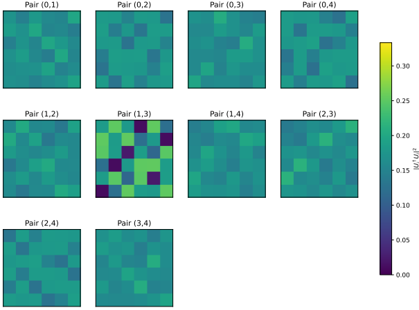
Figure 2: Representative pairwise-loss heatmap for d = 6, n = 5 . The heatmap shows a fully defective structure with all pairs having nonzero loss.
