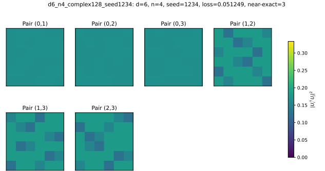
Figure 1: Representative pairwise-loss heatmap for d = 6 , n = 4 . The heatmap shows a hub-and-triangle structure with three near-zero losses and three nonzero losses.
