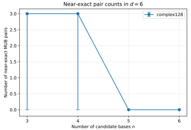
Figure 4: Near-exact MUB pair counts in d = 6 . This plot shows the median number of near-exact MUB pairs with corresponding ranges across five seeds. Near-exact pairs disappear for n \geq 5 under the primary tolerance, coinciding with a transition to fully defective observed configurations.
