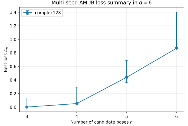
Figure 3: Best AMUB loss summary in d = 6 . This plot shows the median best loss with min-max range across five seeds. The AMUB loss increases with n .
