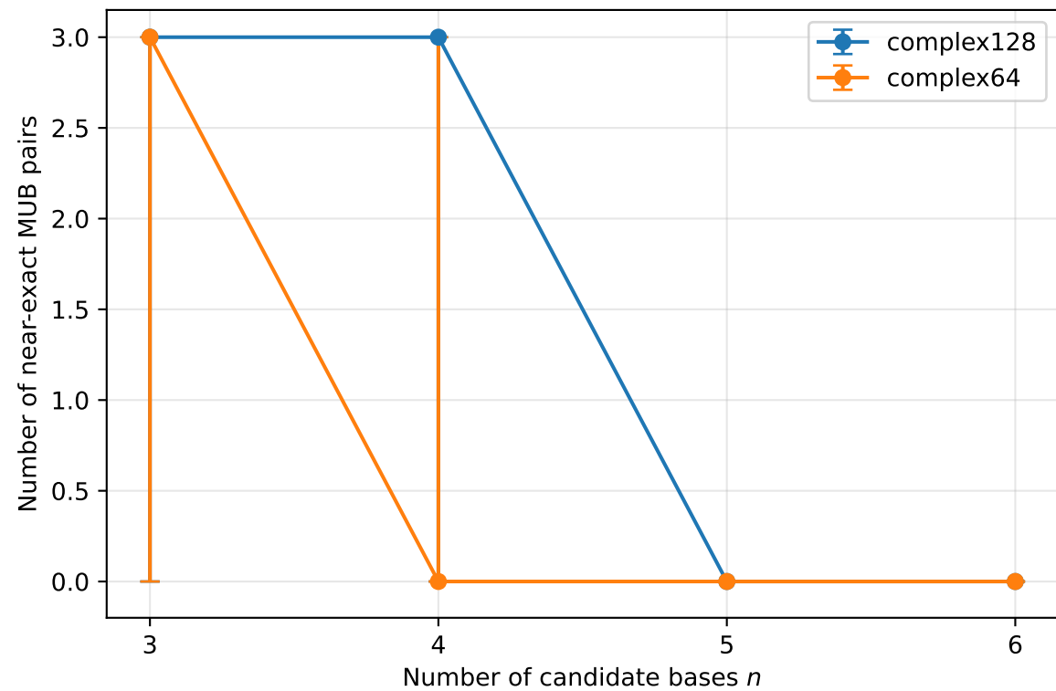
Near-exact pair counts in d = 6
