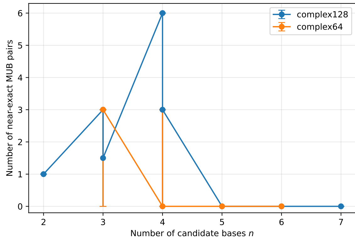
Near-exact pair counts in d = 3
