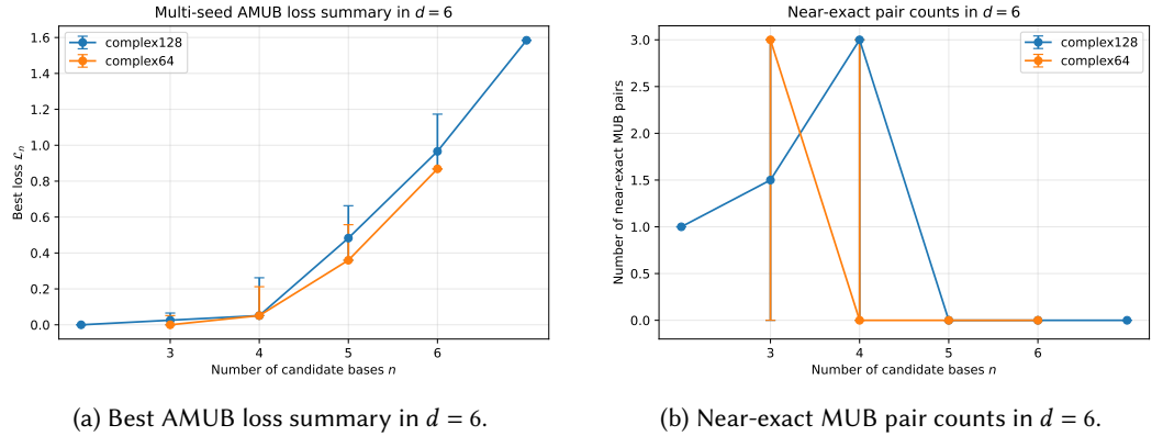
Fig. 2. Multi-seed AMUB optimization summaries in dimension d = 6 . Left: median best loss with min-max range across five seeds. Right: median number of near-exact MUB pairs with corresponding ranges. In the reported campaigns, near-exact pairs disappear for n \geq 5 under the primary tolerance, coinciding with a transition to fully defective observed configurations.
