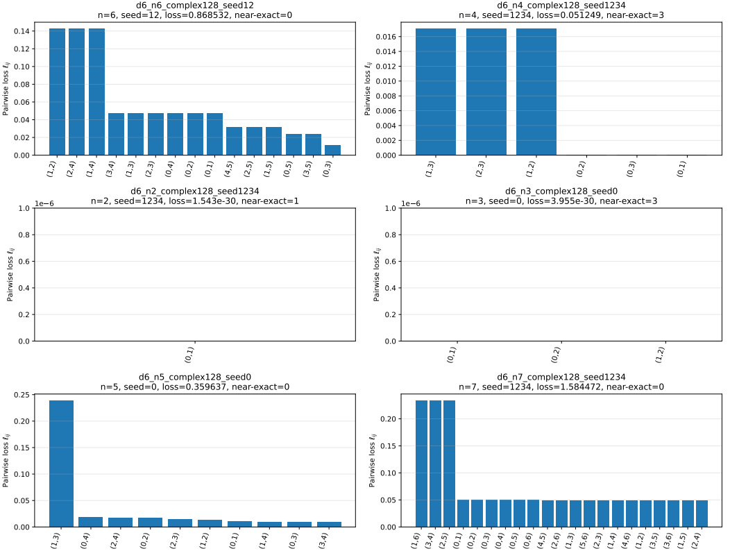
Fig. 3. Sorted pairwise AMUB loss spectra for representative complex128 configurations. Each bar corresponds to one pairwise contribution \ell_{ij} . The exact n = 3 representative has pairwise losses at numerical zero, the defective n = 3 representative has three approximately equal nonzero losses, the n = 4 representative exhibits three near-zero losses and three equal defective losses, and the n = 5 and n = 6 representatives have no zero pairwise losses.
