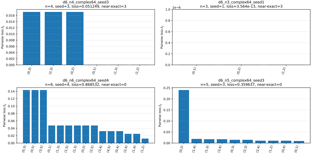
Fig. 4. Sorted pairwise AMUB loss spectra for representative complex64 configurations. Machine-zero losses below the display tolerance are shown as zero for visualization only; raw values are retained in the saved figure-data artifact. The figure illustrates that the main transition to fully defective configurations for n = 5 and n = 6 persists in complex64, while the sampled basins and near-exact classifications differ from the complex128 reference campaign.
