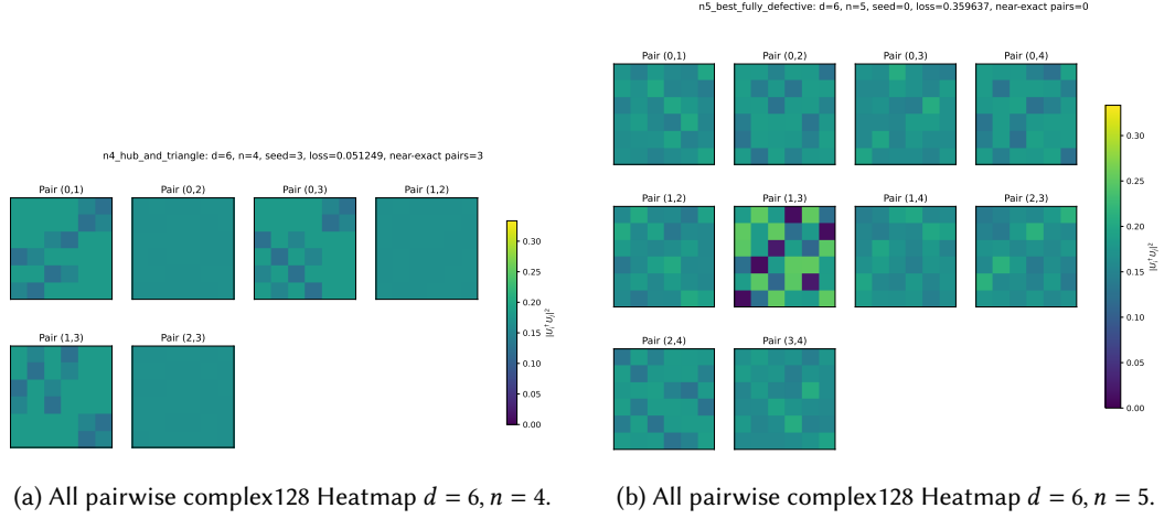
Fig. 1. Representative pairwise-loss heatmaps for n = 4 and n = 5 in dimension six. The n = 4 heatmap shows a hub-and-triangle structure with three near-zero losses and three nonzero losses, while the n = 5 heatmap shows a fully defective structure with all pairs having nonzero loss.
