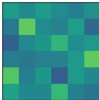
Pair (2,3)
