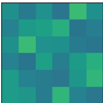
Pair (3,4)
