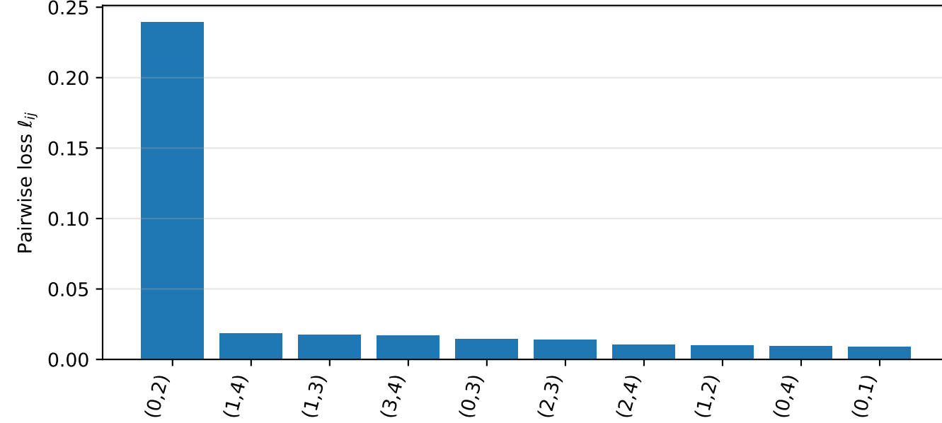
n5_best_fully_defective n=5, seed=3, loss=0.359637, near-exact=0
