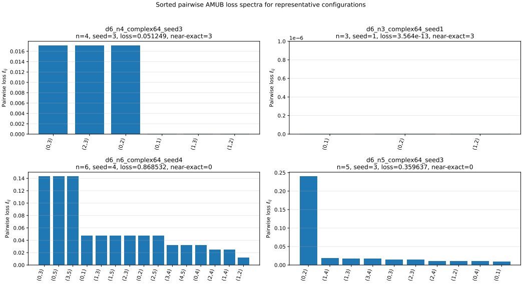
Fig. 4. Sorted pairwise AMUB loss spectra for representative complex64 configurations. Machine-zero losses below the display tolerance are shown as zero for visualization only; raw values are retained in the saved figure-data artifact. The figure illustrates that the main transition to fully defective configurations for n = 5 and n = 6 persists in complex64, while the sampled basins and near-exact classifications differ from the complex128 reference campaign.
