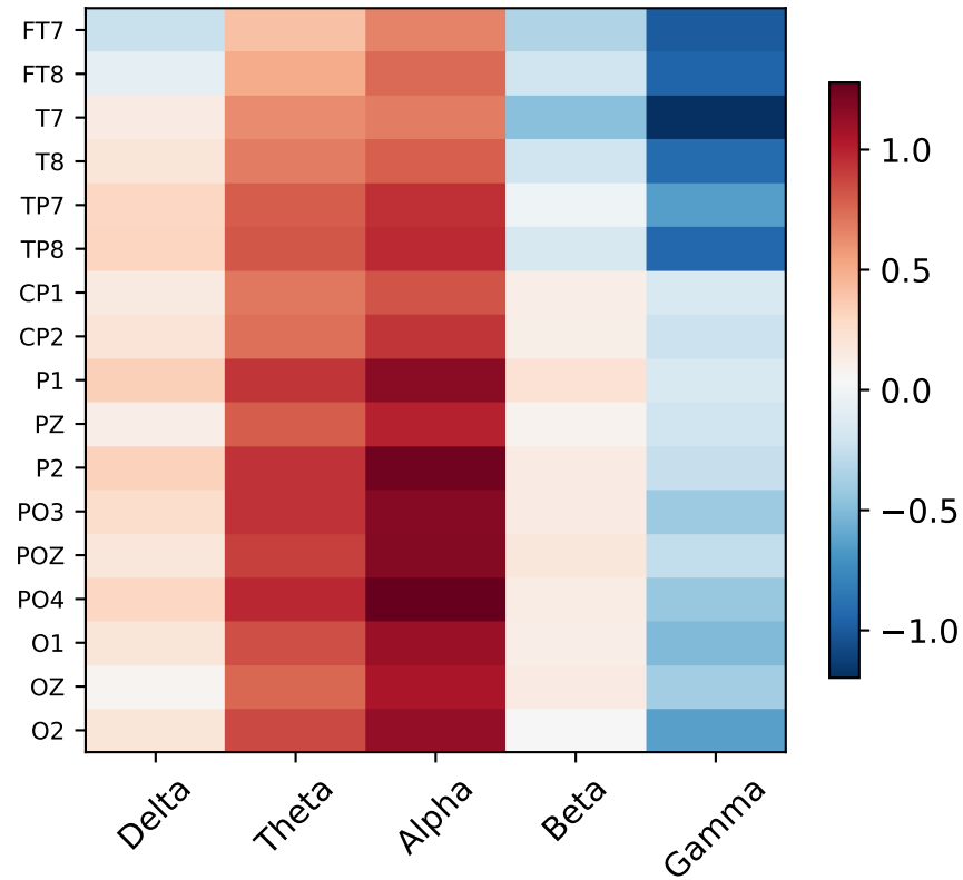
Difference (Drowsy-Alert)
