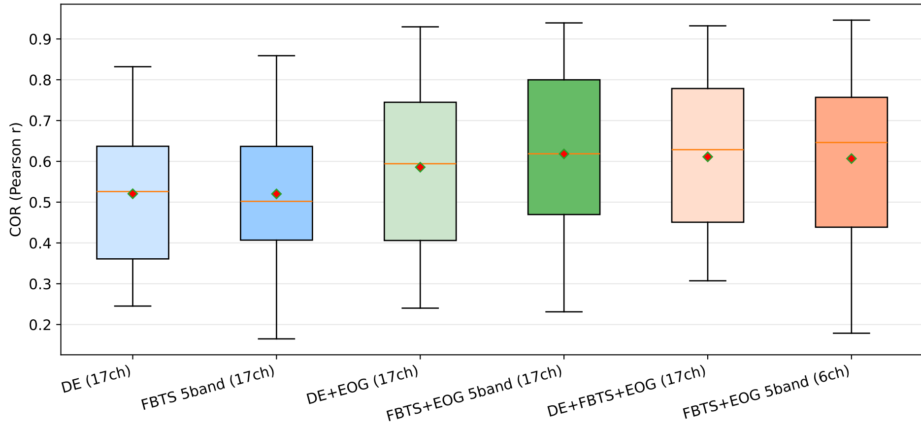
Per-Subject COR Distribution (23 subjects, 5-fold CV)
