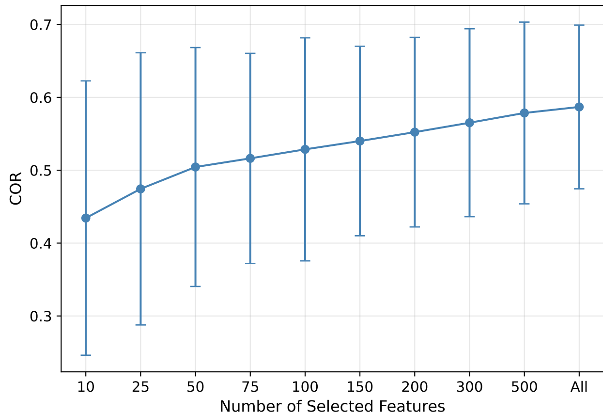
FBTS Feature Dimension Ablation (5 subjects)
