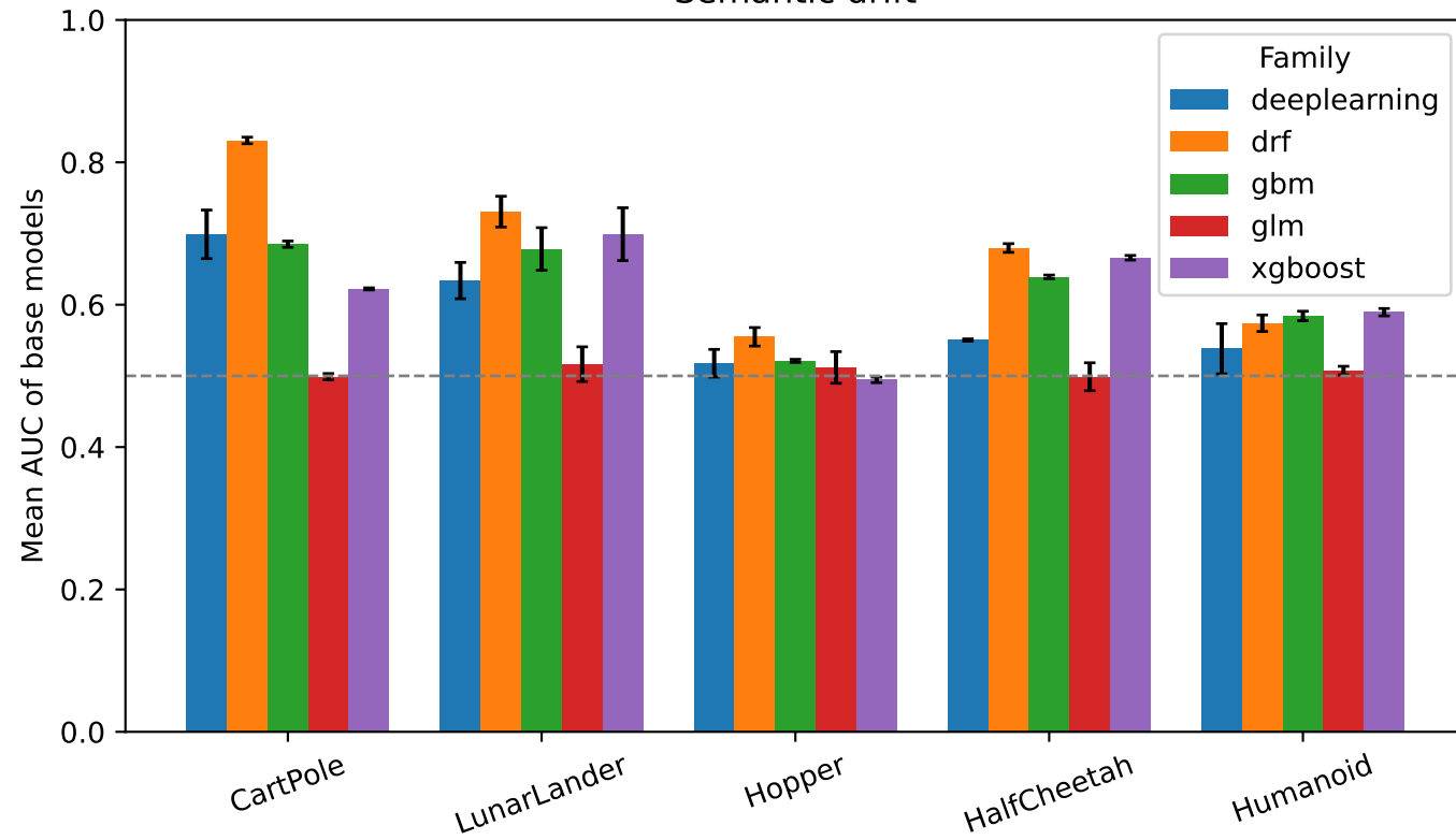
Semantic drift
