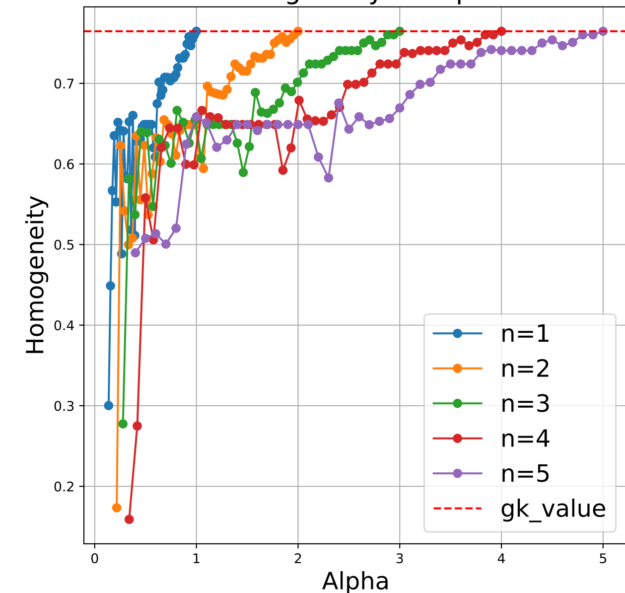
Homogeneity vs Alpha
