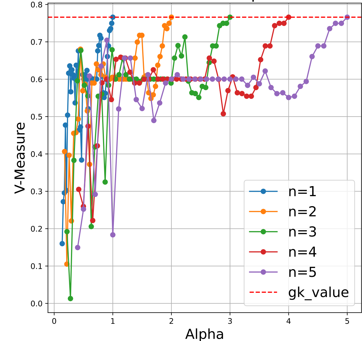
V-Measure vs Alpha
