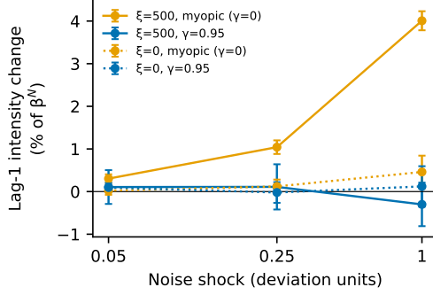
Fig. 8. Noise-shock responses with shared Q-tables. At \xi = 500 the myopic placebo (orange, solid) ignores small shocks and reacts increasingly to larger ones, the pattern read as a price trigger, although with \gamma = 0 it has no reason to punish.
