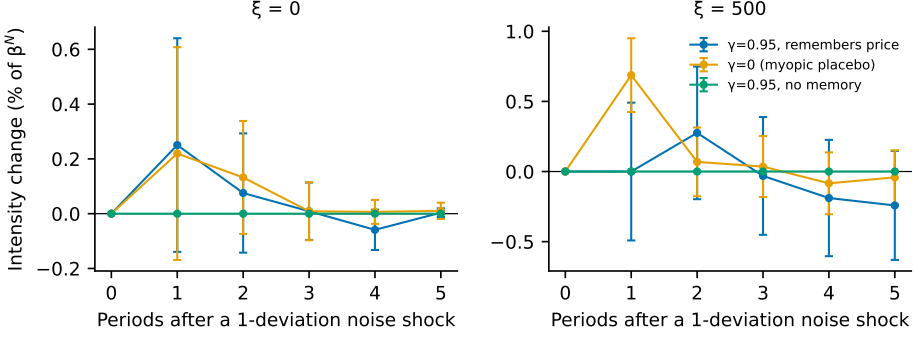
Fig. 4. Noise-shock impulse responses in the Dou et al. [2025] calibration with separate Q-tables. A noise-trader shock equal to one best-response deviation hits at lag 0; lines show the change in per-trader intensity in % of \beta^N . Under price-trigger strategies intensity would jump at lag 1.
