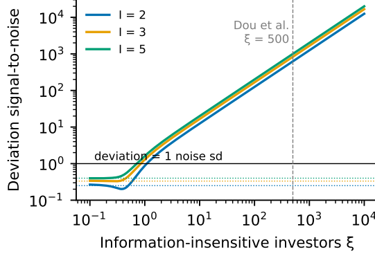
Fig. 6. Signal-to-noise ratio of a one-period best-response deviation from the collusive intensity (order-flow change per unit of v/\sigma_v , in noise standard deviations), as a function of the mass of information-insensitive investors ( \sigma_v = 1 , \sigma_u = 0.1 , \theta = 0.1 ). Dotted lines: the \xi = 0 values (I - 1)/(2I) . Deviations become visible above noise only once \xi exceeds about one; at the Dou et al. [2025] calibration they are several hundred noise standard deviations large.
