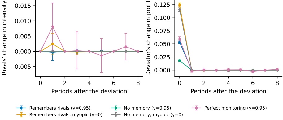
Fig. 7. Rival-deviation test. Left: change in rivals' trading intensity after trader 1 plays its one-period best response at lag 0. Right: the deviator's change in profit. Paired simulations with common random numbers; 95% confidence intervals.
