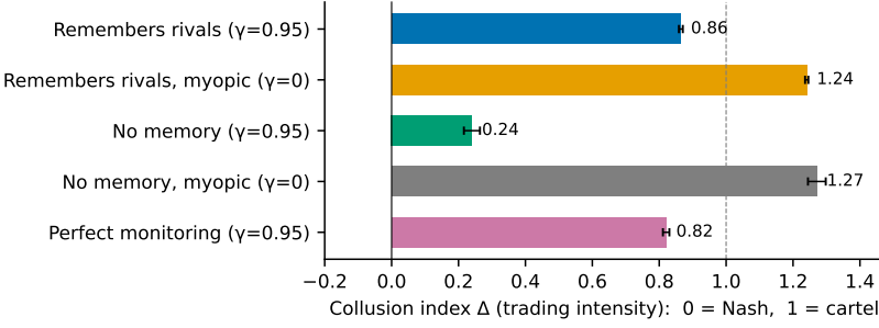
Fig. 3. Collusion index (trading intensity) by condition. The myopic placebo, which cannot collude, scores beyond the cartel.
