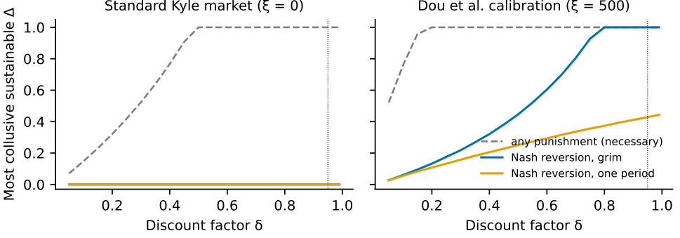
Fig. 1. Most collusive outcome (in units of \Delta intensity) that trigger strategies can sustain, by discount factor. Solid lines: static-Nash reversion with the best threshold, forever (grim) or for one period (the harshest phase a memory-one strategy can run). Dashed: the necessary condition of Proposition 3.4, which no scheme can beat. Dotted: \delta = 0.95 , used in all experiments. Left: \sigma_u = 1 , 5 values; right: Dou et al. [2025]’s calibration, 10 values.
