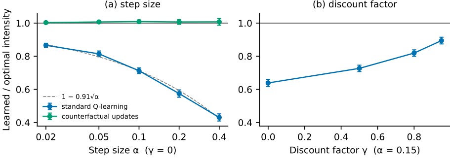
Fig. 2. Pruning without a game. One informed trader facing a fixed price rule ( I = 1 , no memory, 3 \times 10^5 periods, 100 runs per point, 95% CIs). (a) With \gamma = 0 , standard Q-learning under-trades by about 0.91\sqrt{\alpha} (dashed); counterfactual updates learn the optimal order at every step size. (b) At \alpha = 0.15 the shortfall shrinks as the discount factor rises.
