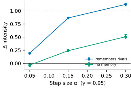
Fig. 9. The collusion index rises with the constant step size \alpha (standard Kyle market, \gamma = 0.95 , 200 markets per point). No configuration punishes deviations.
