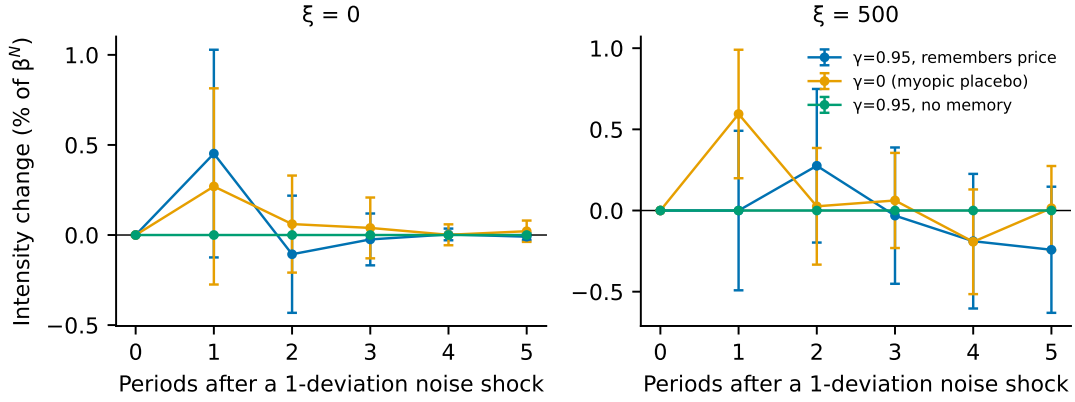
Figure 5: Noise-shock impulse responses in the Dou et al. [12] calibration with separate Q-tables. A noise-trader shock equal to one best-response deviation hits at lag 0; lines show the change in per-trader intensity in % of \beta^N . Under price-trigger strategies intensity would jump at lag 1.
