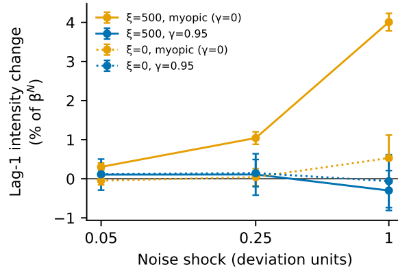
Figure 6: Noise-shock responses with shared Q-tables. At \xi = 500 the myopic placebo (orange, solid) ignores small shocks and reacts increasingly to larger ones, the pattern read as a price trigger, although with \gamma = 0 it has no reason to punish.
