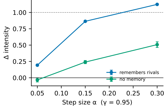
Figure 7: The collusion index rises with the constant step size \alpha (standard Kyle market, \gamma = 0.95 , 200 markets per point). No configuration punishes deviations.
