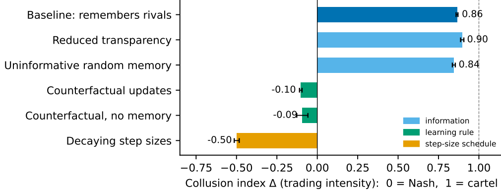
Figure 8: Interventions in the standard Kyle market. Treatments that change what traders observe leave the outcome unchanged; treatments that change how they learn move it to, or past, competition.
