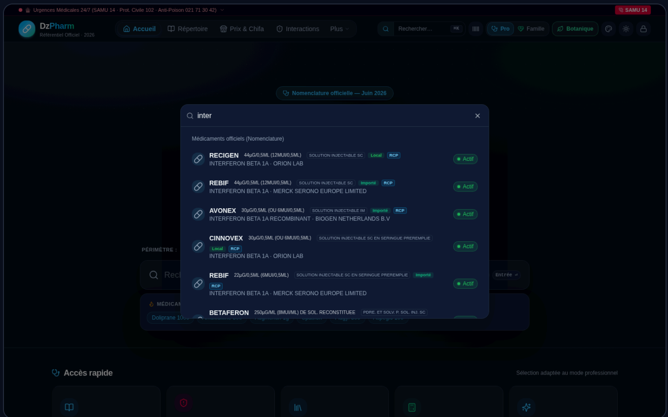
Figure 11.2 — Palette with «inter» typed. Results show BOTH Interferon medications from the 9,555-AMM database AND the «Contrôle d'interactions médicamenteuses» command — the palette searches two datasets in parallel and merges results. This is genuinely uncommon and useful.
