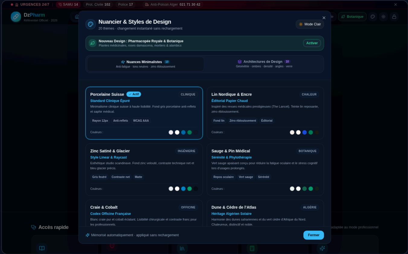
Figure 58.1 – Nuancier dialog showing 20 themed palettes. Current: «Porcelaine Suisse» (CLINIQUE, Actif). Categories: Nuances Minimalistes (10), Architectures de Design (10), plus «Pharmacopée Royale & Botanique» new design mode.
