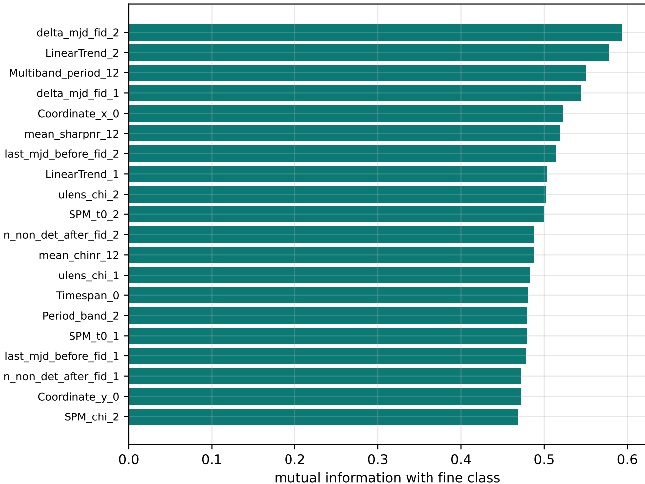
Top-20 features by mutual information (train)
