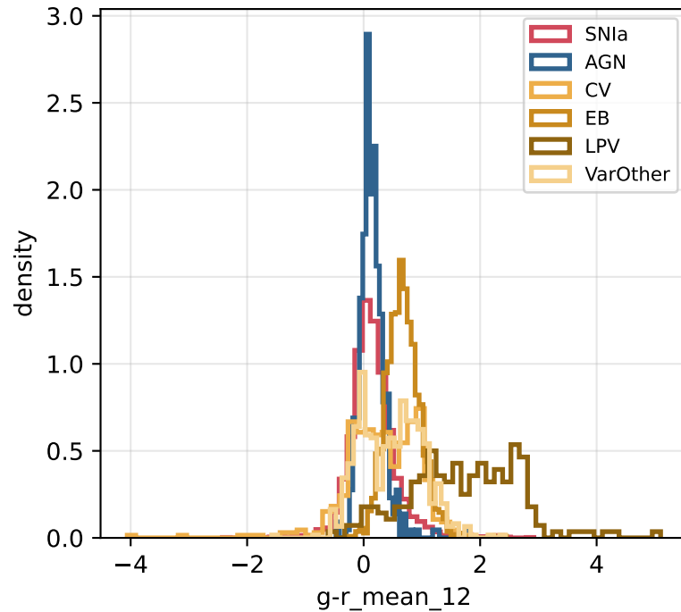
Class separation on headline features (train, 6-class subset)
