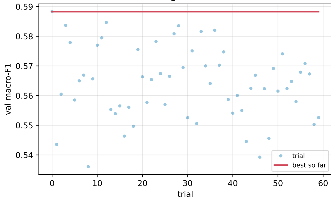
BalancedRF
