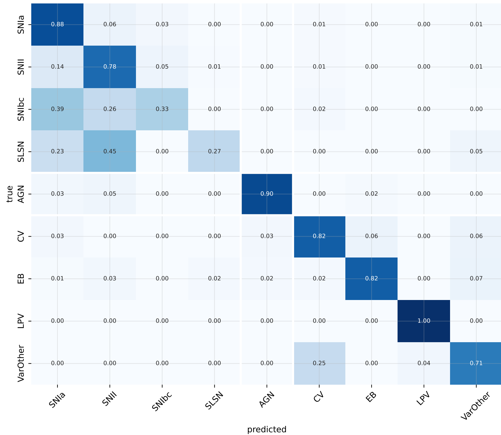
Flat XGBoost (macro-F1 0.705)
