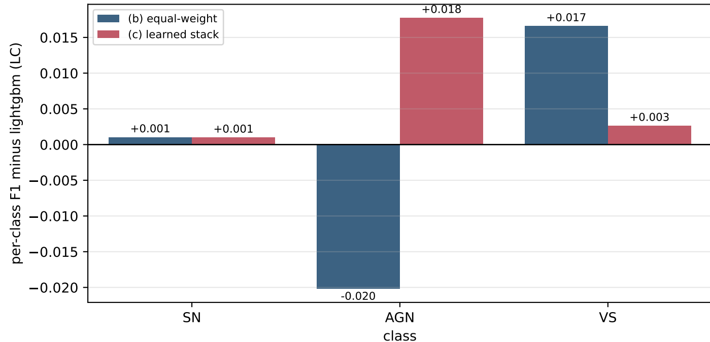
Where fusion helps and where it hurts, by class
