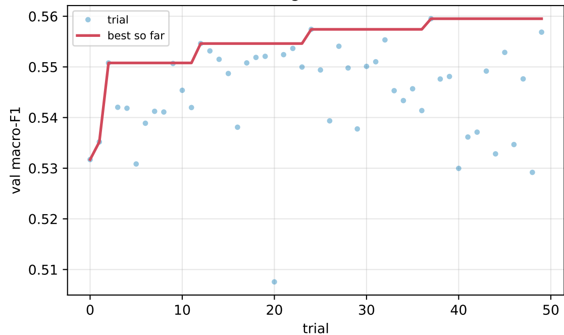
BalancedRF
