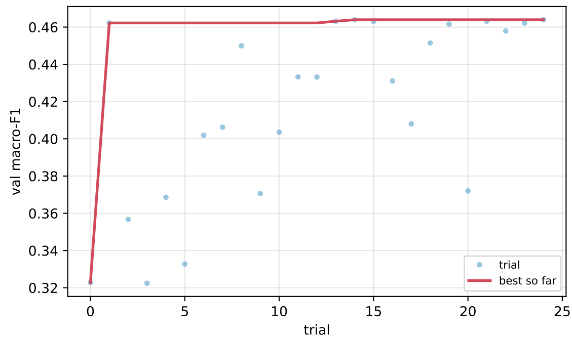
BalancedRF
