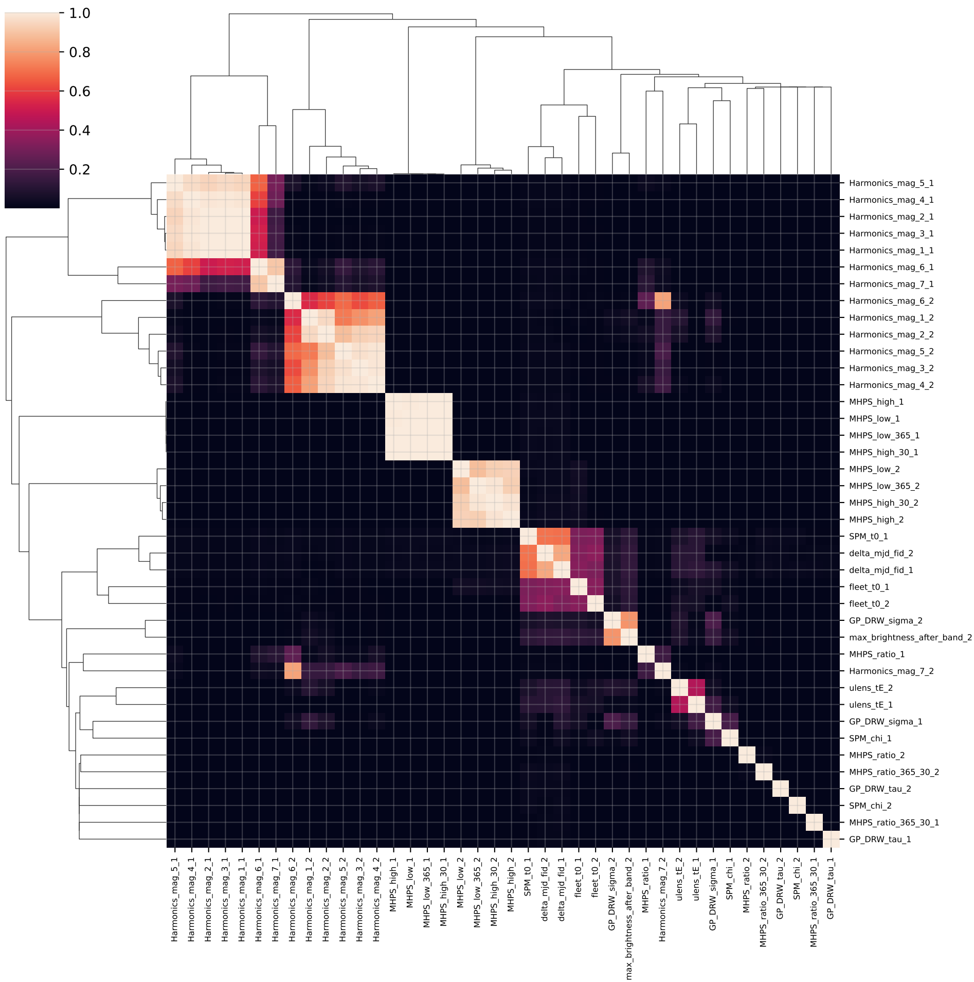
Correlation clustering of 40 highest-variance features
