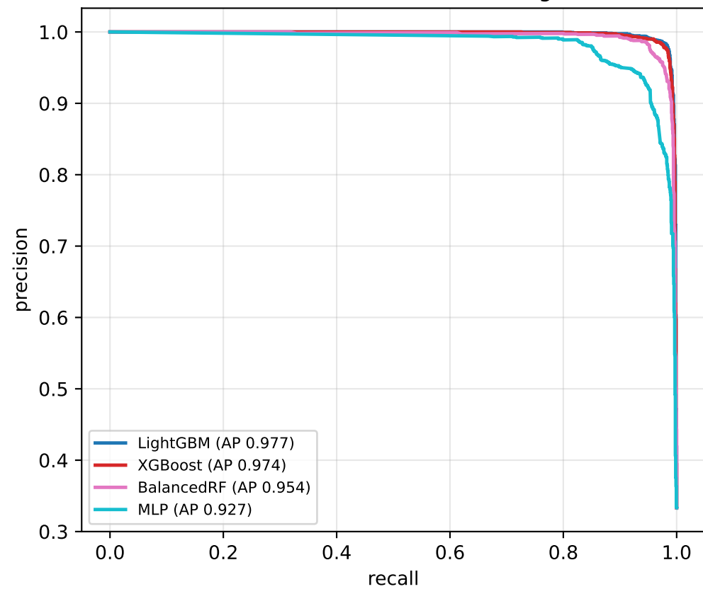
Precision-recall (micro-average)
