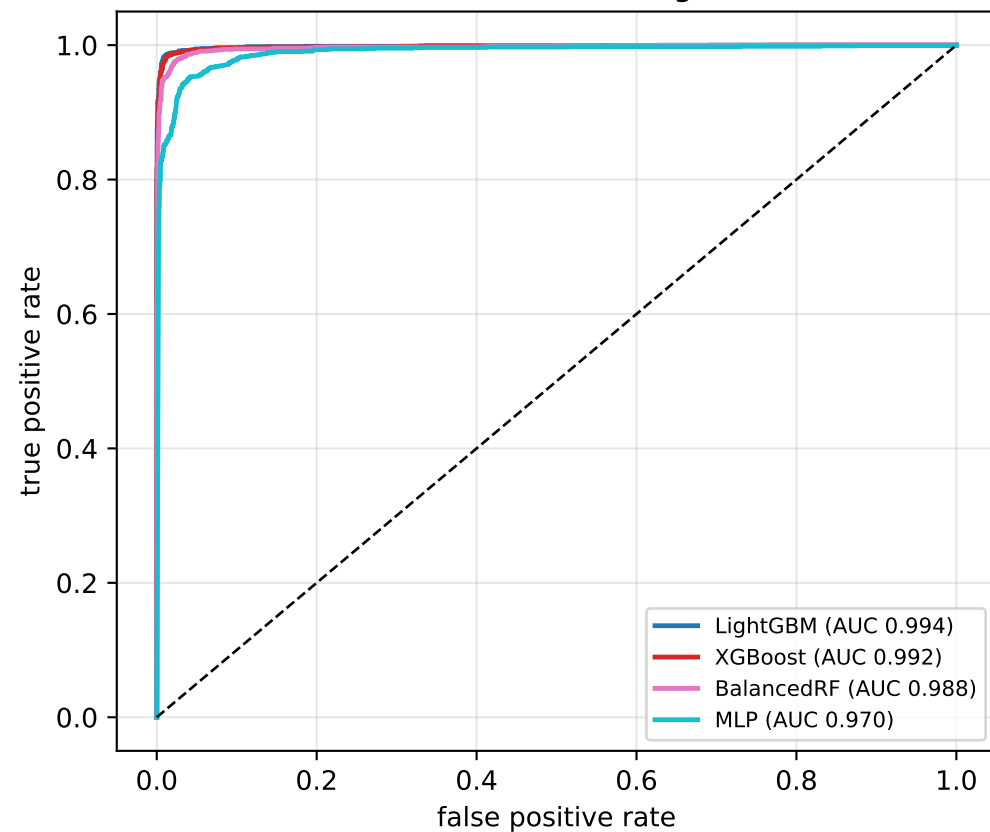
ROC (micro-average)
