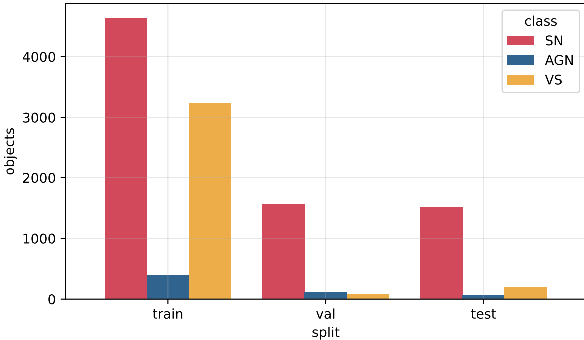
Coarse class balance per temporal split (stamps)
