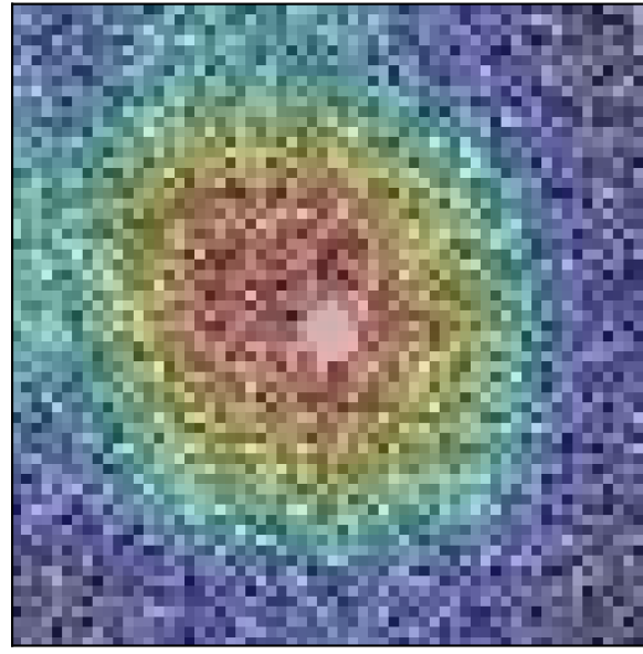
ResNet-18
