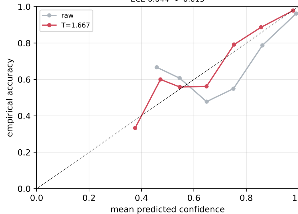
EfficientNet-B0 (stamp) — val ECE 0.044 -> 0.015
