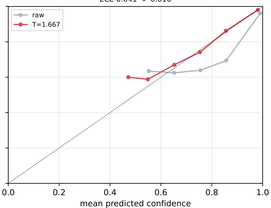
EfficientNet-B0 (stamp) — test ECE 0.041 -> 0.010
