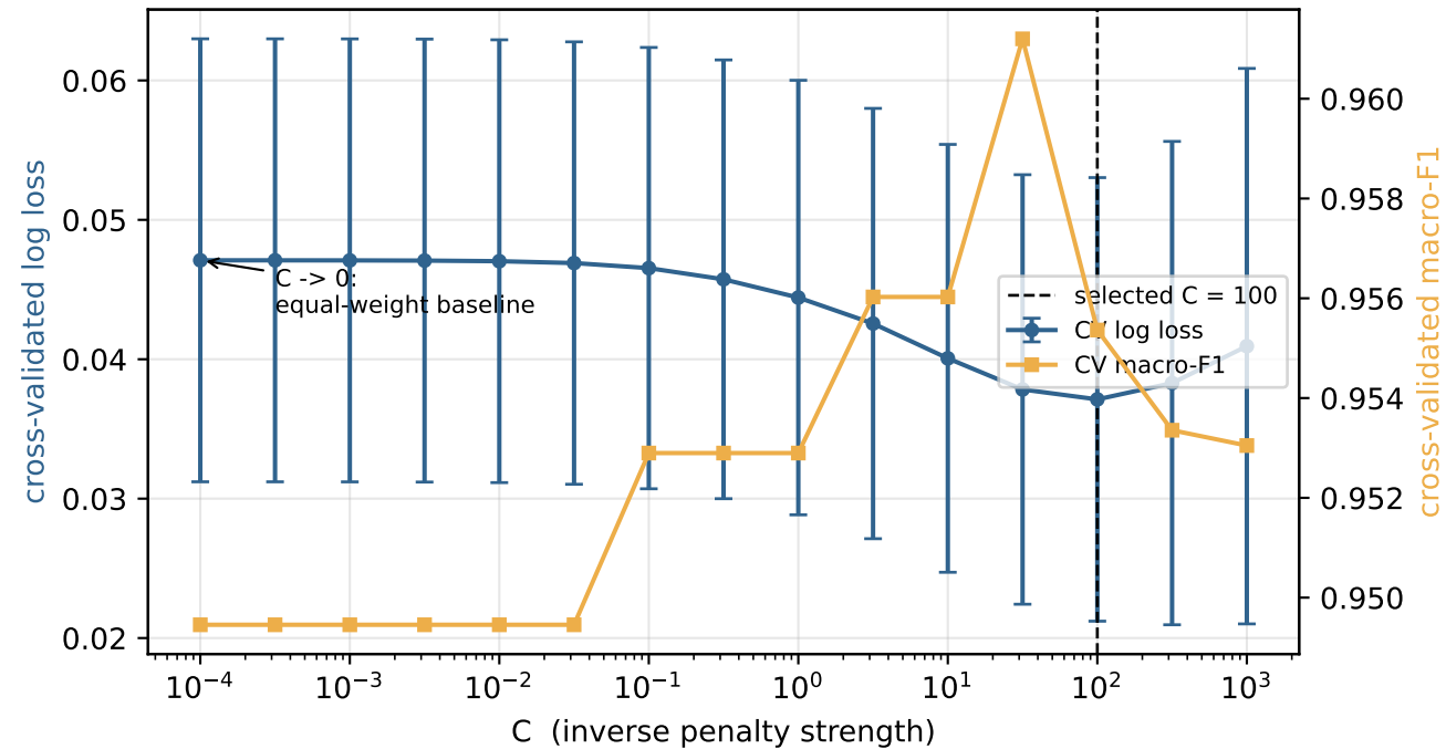
Regularisation path: the equal-weight baseline is the C \rightarrow 0 limit
