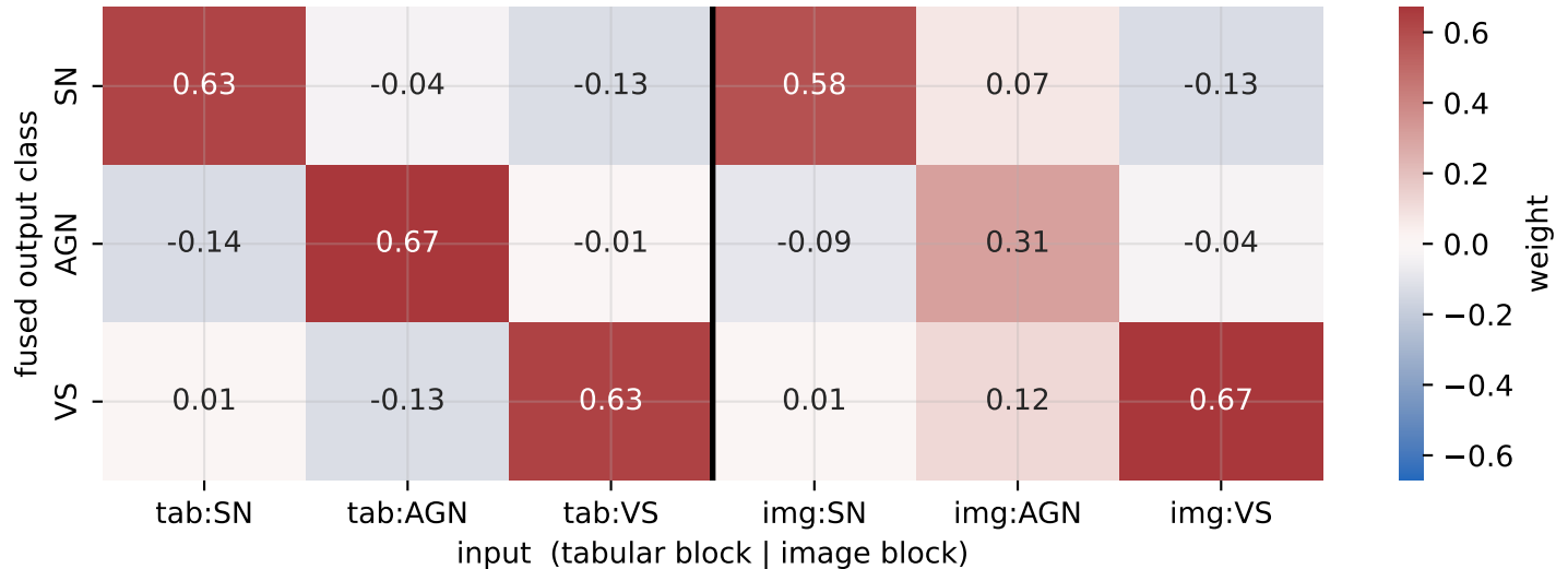
Learned fusion weights W ( C = 100 ; equal-weight prior = 0.5 on the diagonals)
