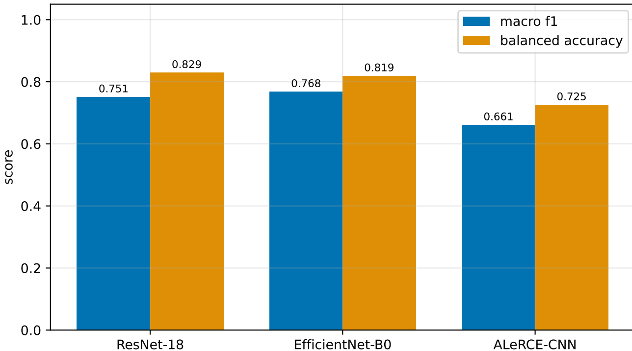
ZTF stamps — architecture comparison (test)
