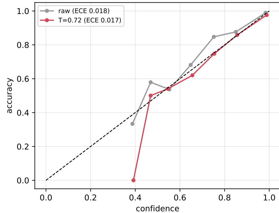
ResNet-18
