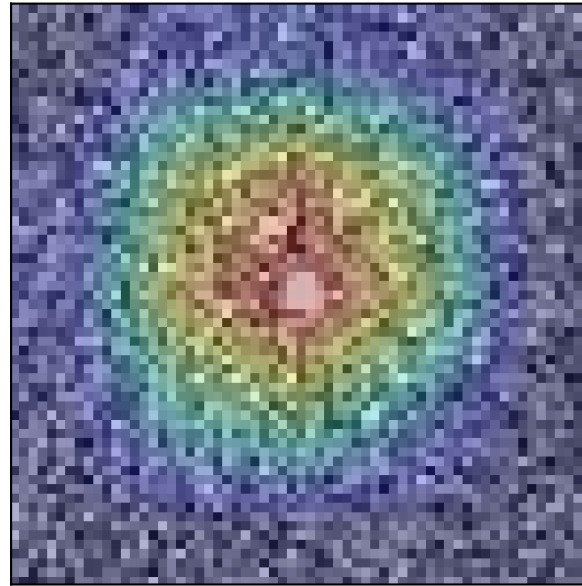
ResNet-18
