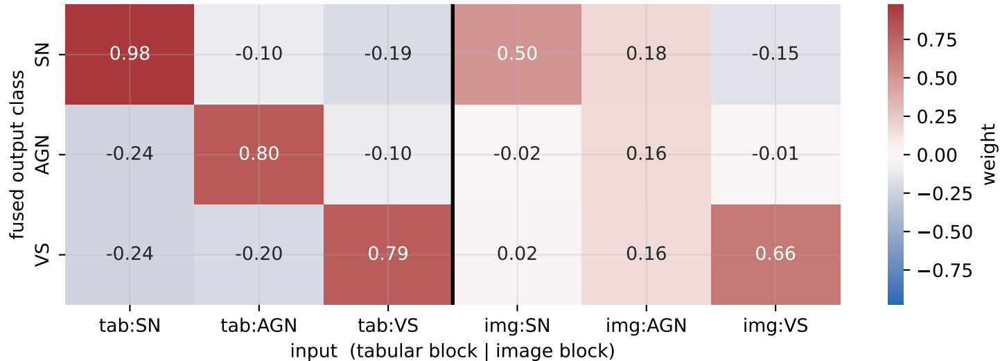
Learned fusion weights W ( C = 1e+03 ; equal-weight prior = 0.5 on the diagonals)
