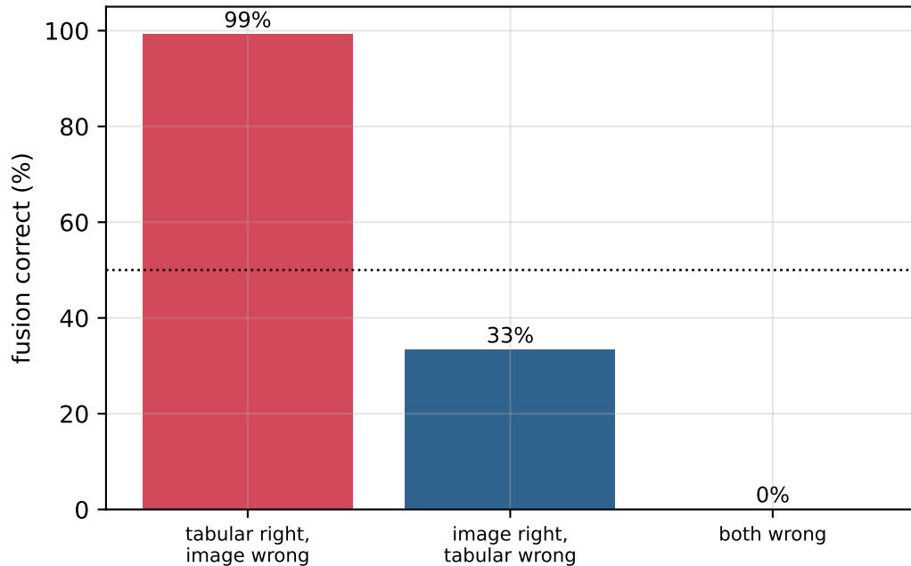
Does the stack pick the right branch when they disagree?
