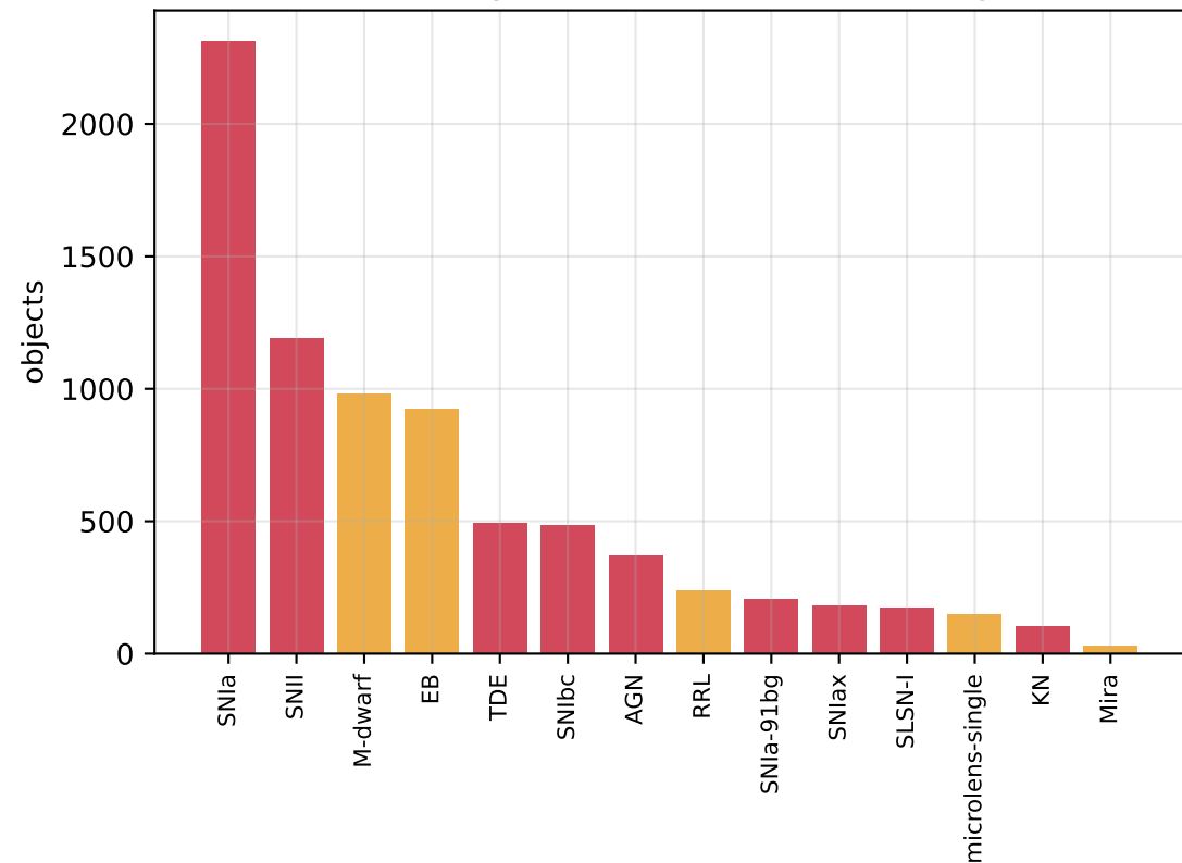
Native classes (yellow=Galactic, red=extragalactic)
