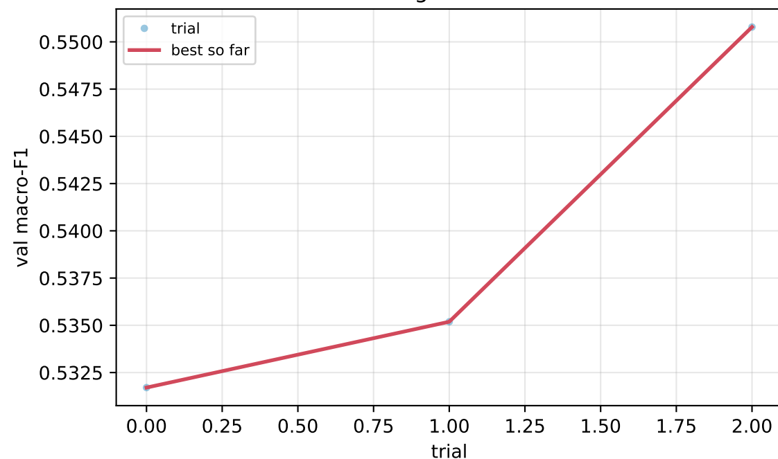
BalancedRF
