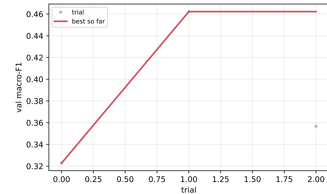
BalancedRF
