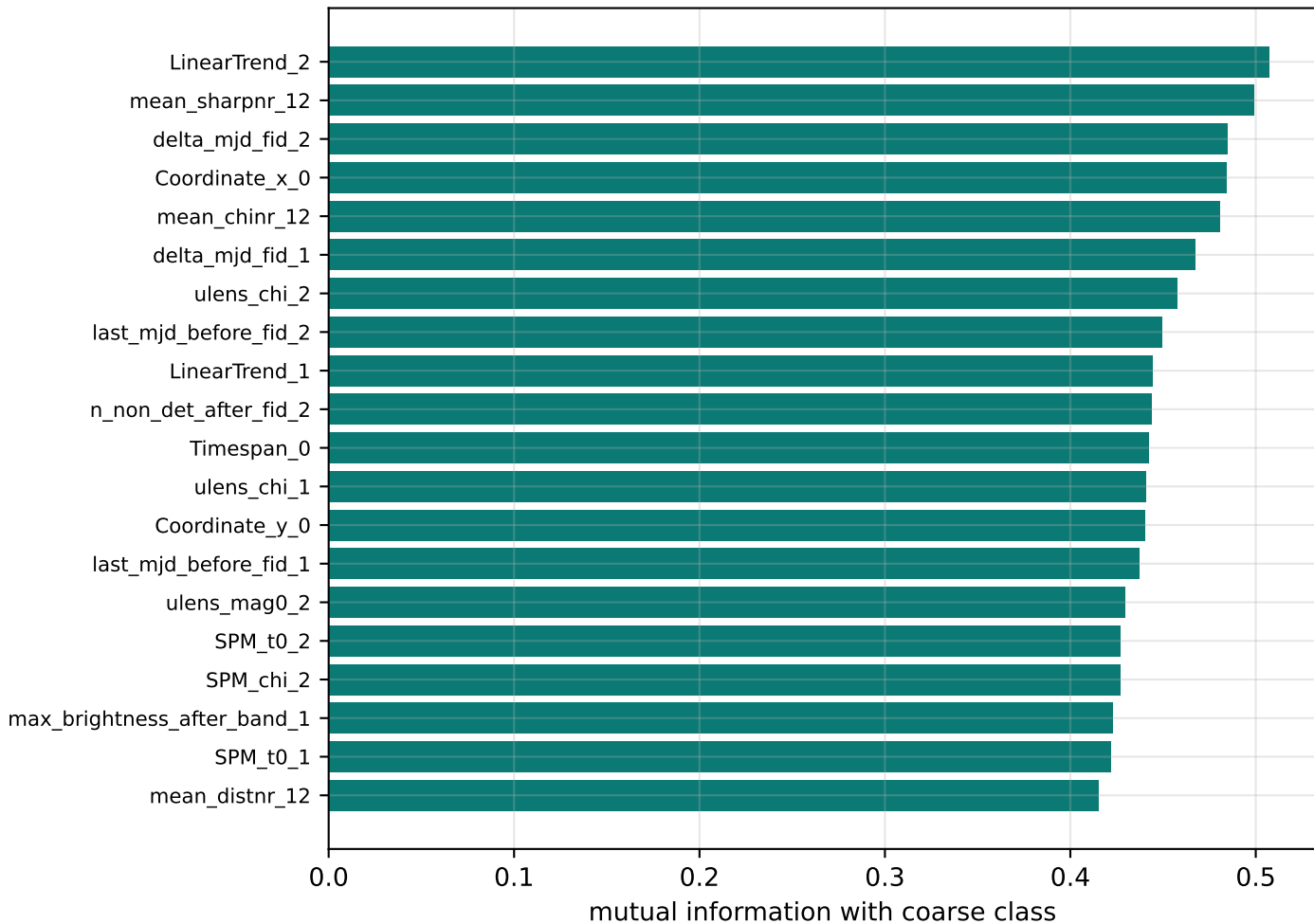
Top-20 features by mutual information (train)
