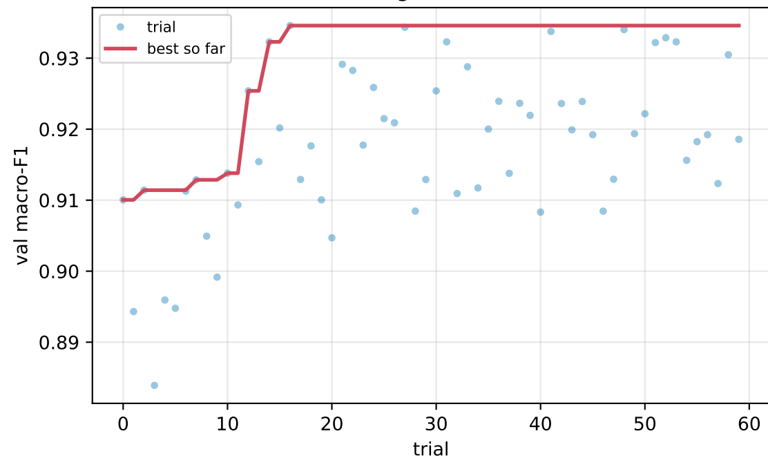
BalancedRF
